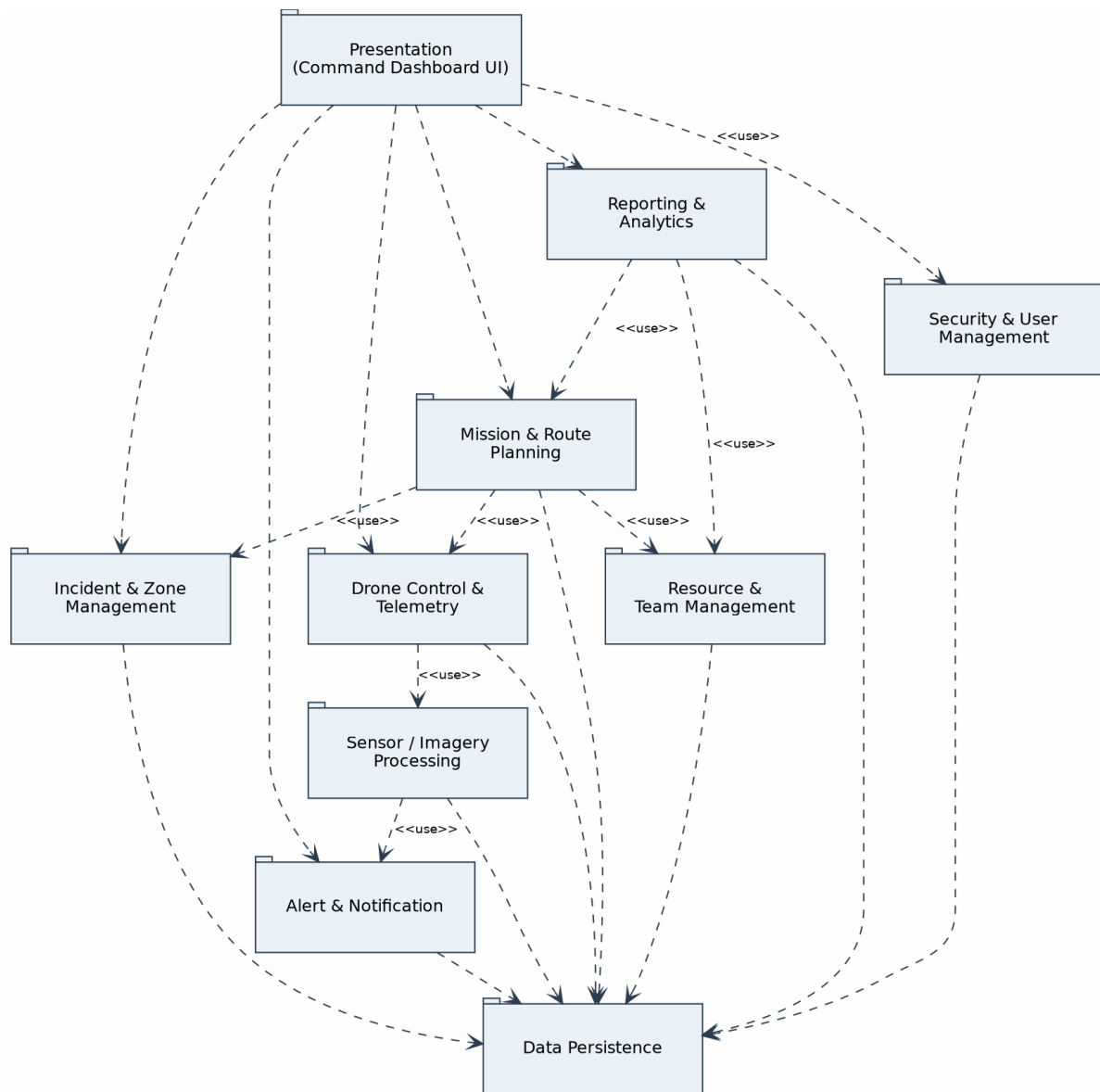
Figure 10.1: Package Diagram - ADDRRS Modules
